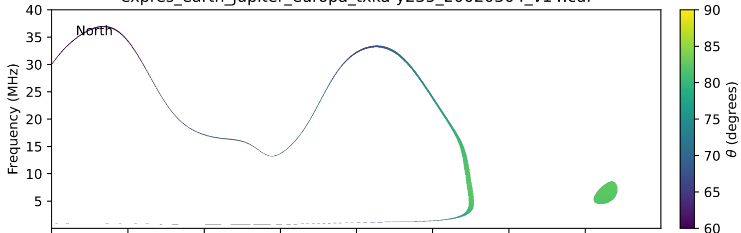
expres_earth_jupiter_europa_txka-y235_20020304_v14.cdf
