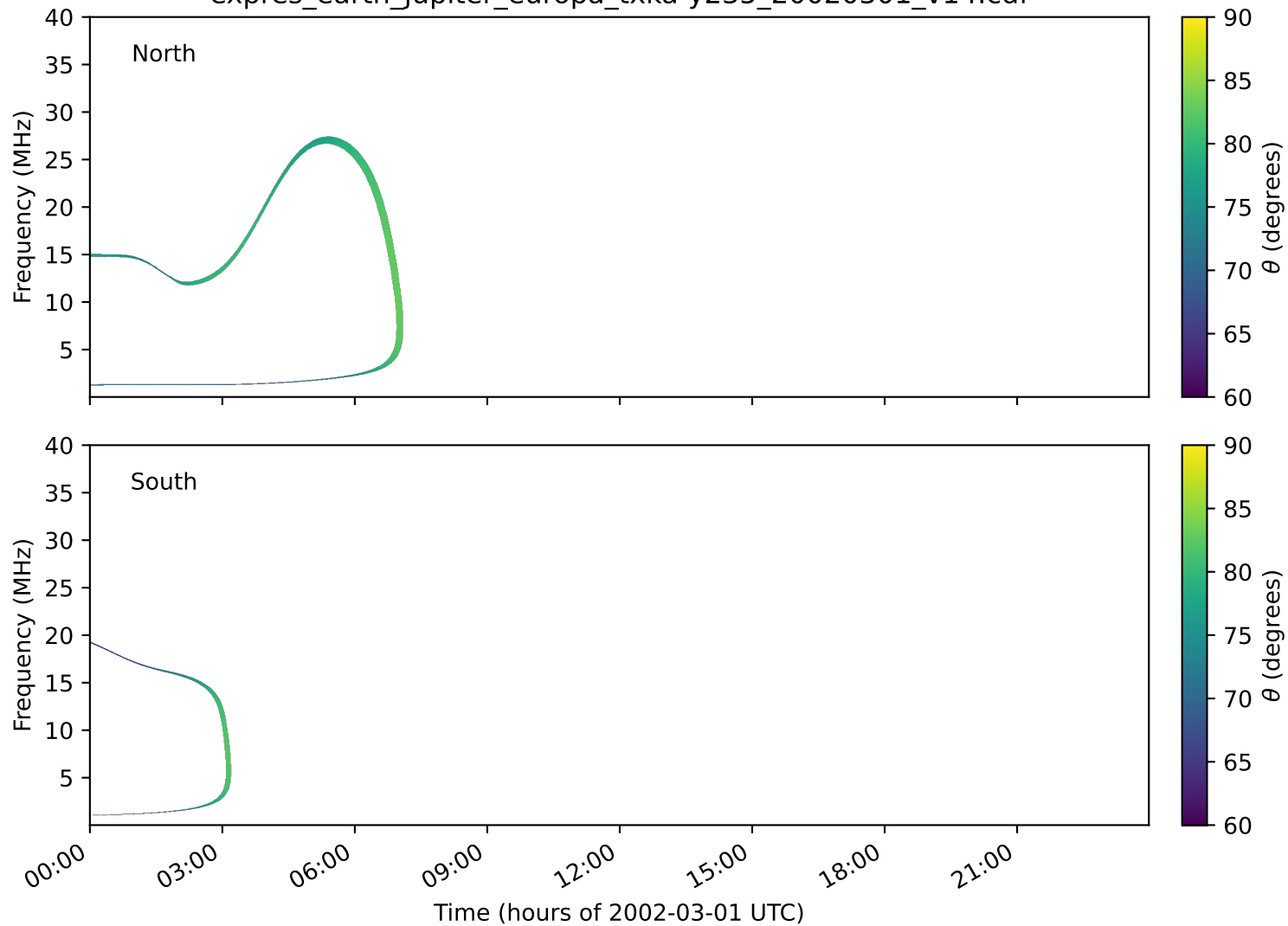
expres_earth_jupiter_europa_txka-y235_20020301_v14.cdf
