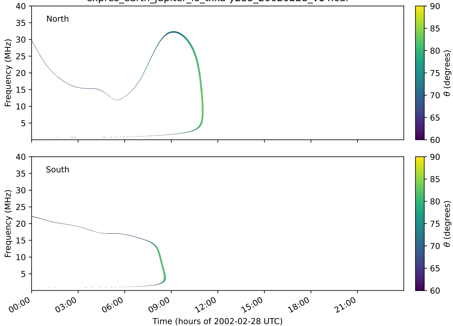
expres_earth_jupiter_io_txka-y235_20020228_v14.cdf
