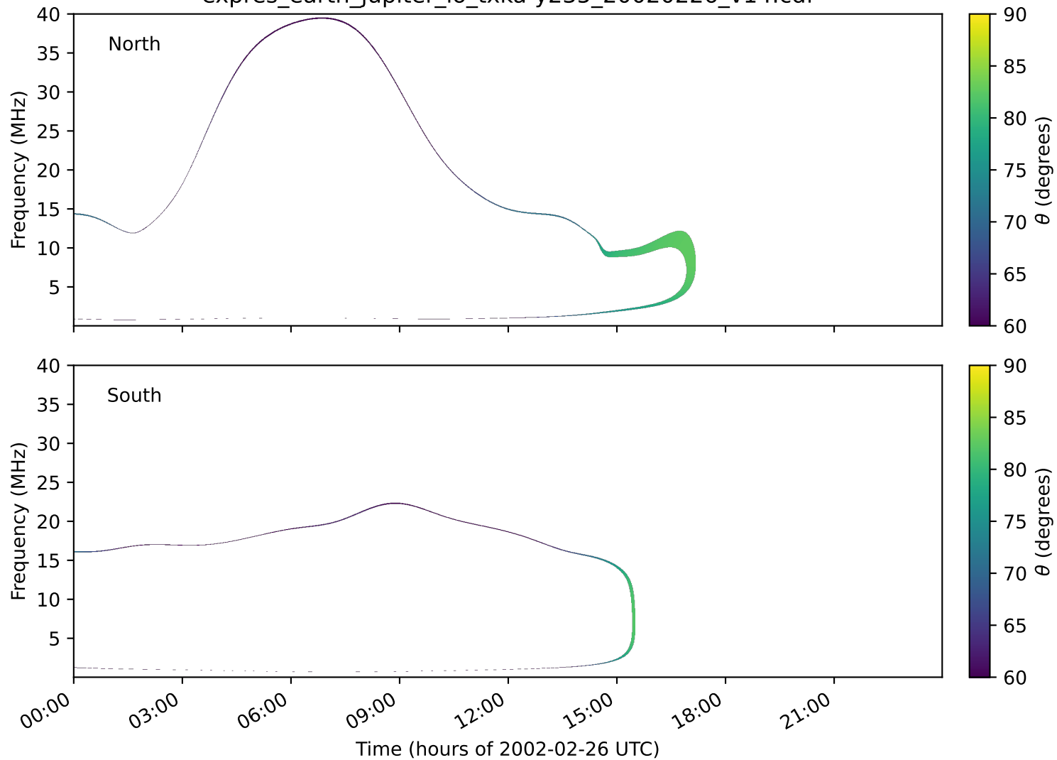
expres_earth_jupiter_io_txka-y235_20020226_v14.cdf
