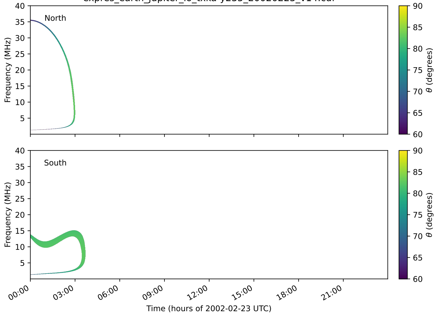
expres_earth_jupiter_io_txka-y235_20020223_v14.cdf
