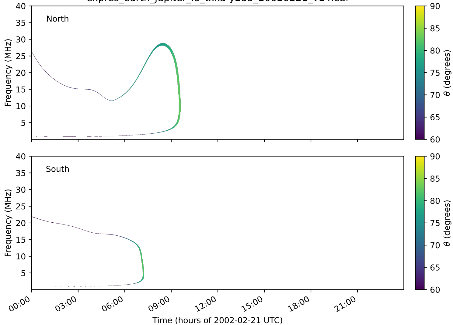
expres_earth_jupiter_io_txka-y235_20020221_v14.cdf
