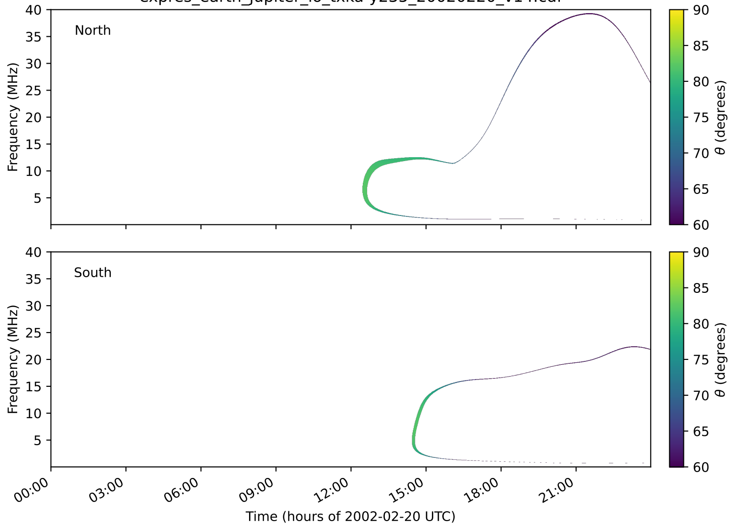
expres_earth_jupiter_io_txka-y235_20020220_v14.cdf
