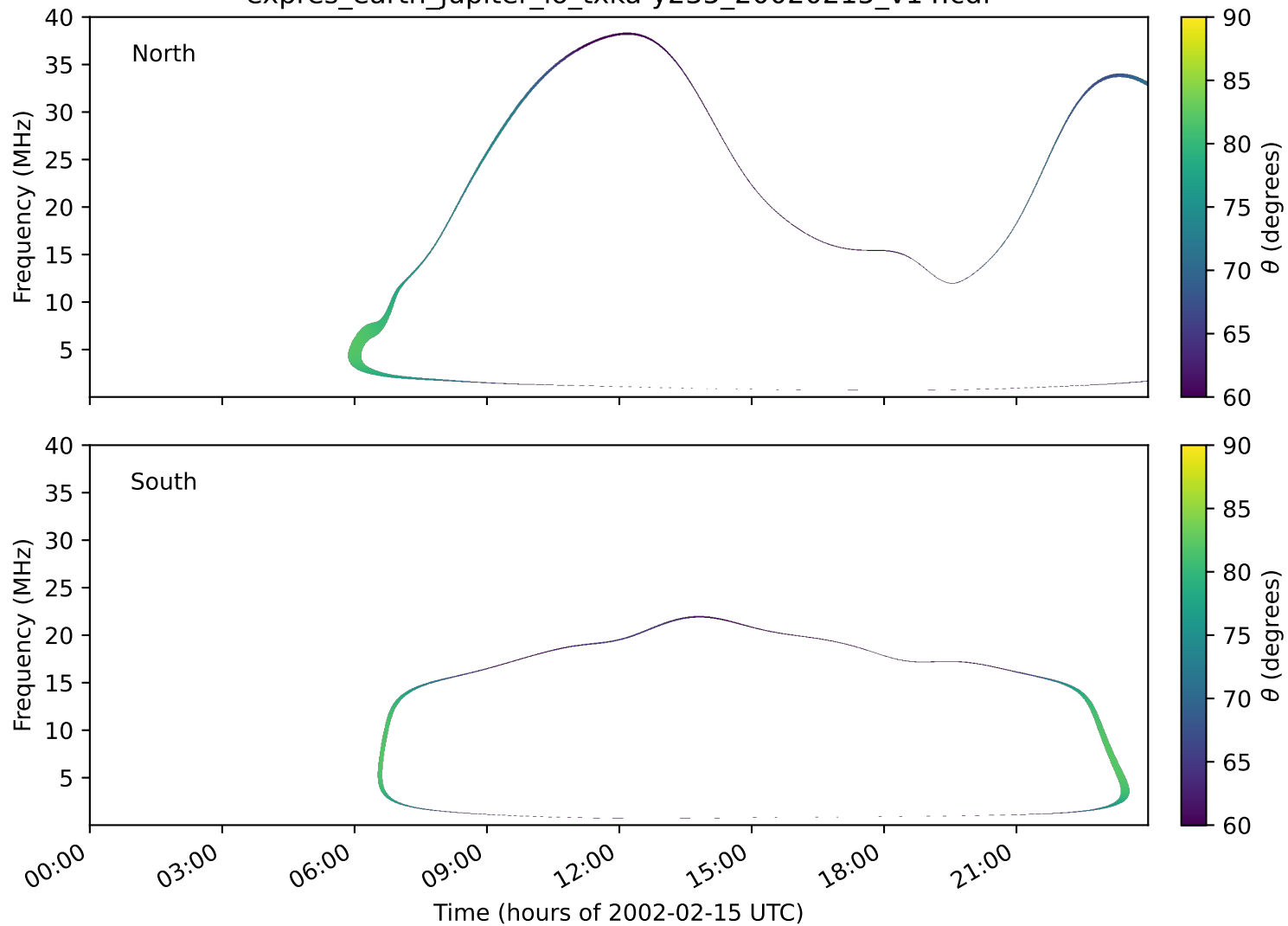
expres_earth_jupiter_io_txka-y235_20020215_v14.cdf
