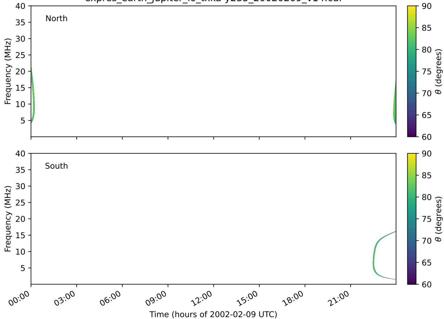
expres_earth_jupiter_io_txka-y235_20020209_v14.cdf
