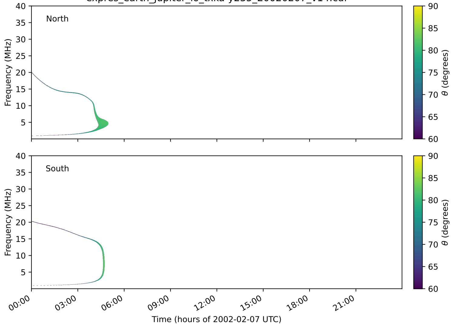
expres_earth_jupiter_io_txka-y235_20020207_v14.cdf
