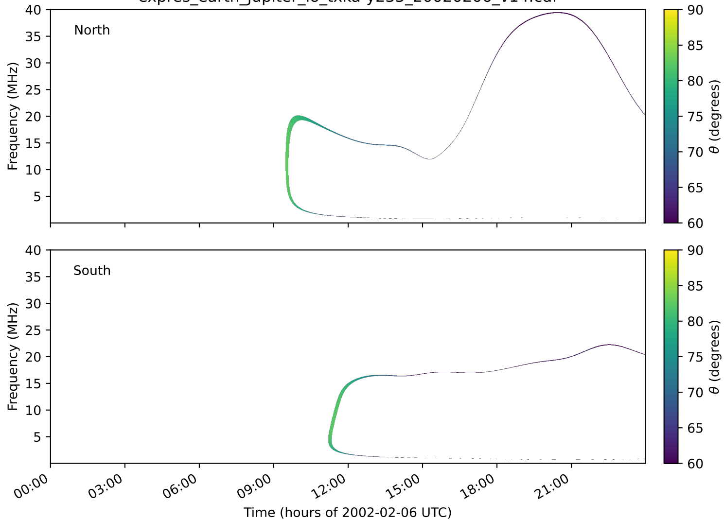
expres_earth_jupiter_io_txka-y235_20020206_v14.cdf
