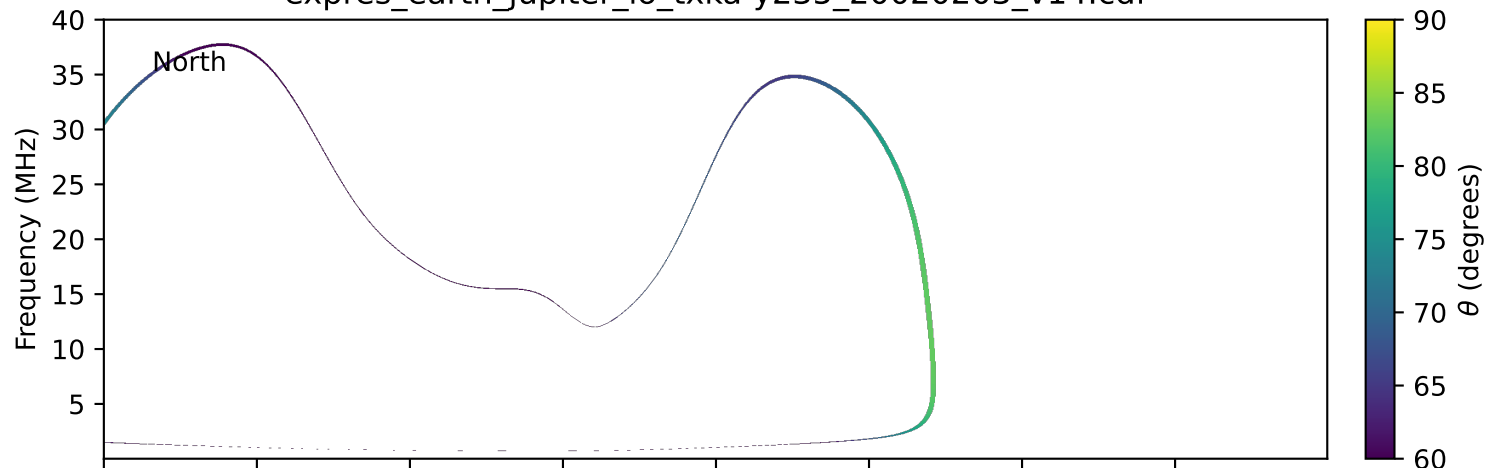
expres_earth_jupiter_io_txka-y235_20020203_v14.cdf
