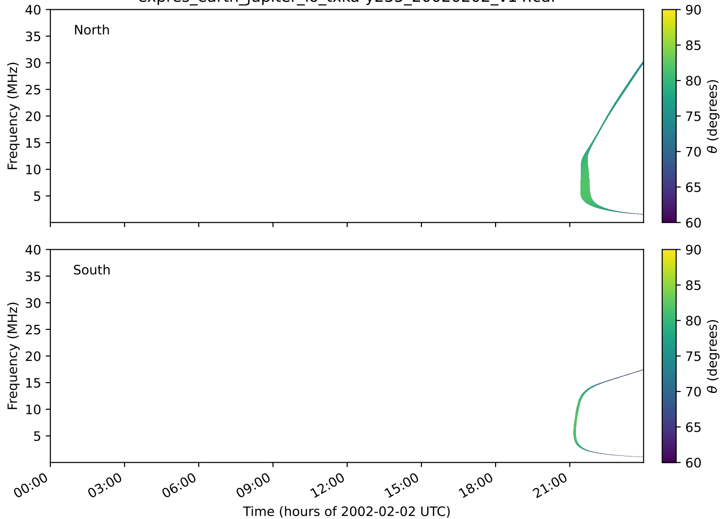
expres_earth_jupiter_io_txka-y235_20020202_v14.cdf
