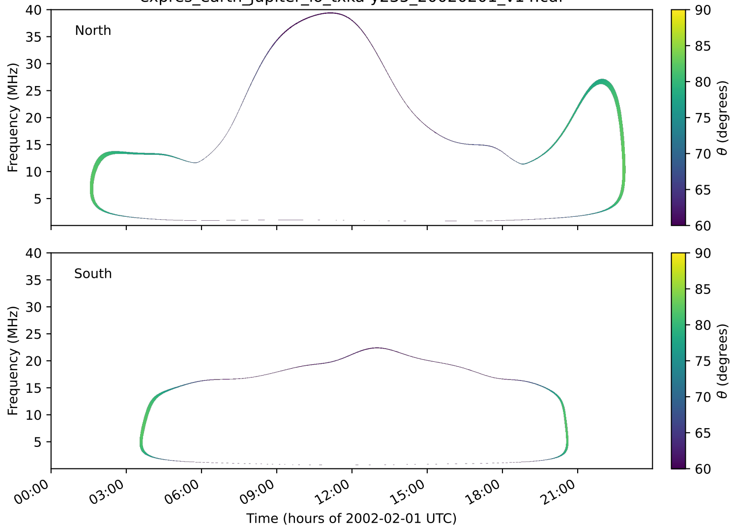
expres_earth_jupiter_io_txka-y235_20020201_v14.cdf
