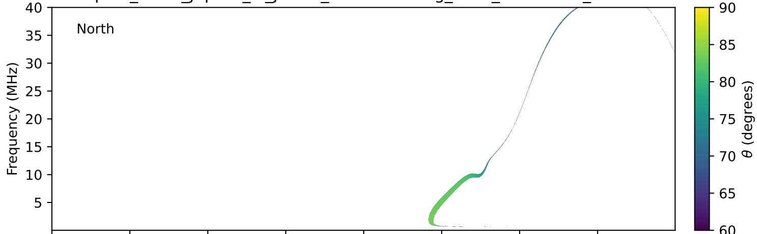
expres_earth_jupiter_io_jrm33_lossc-wid1deg_3kev_20020227_v11.cdf
