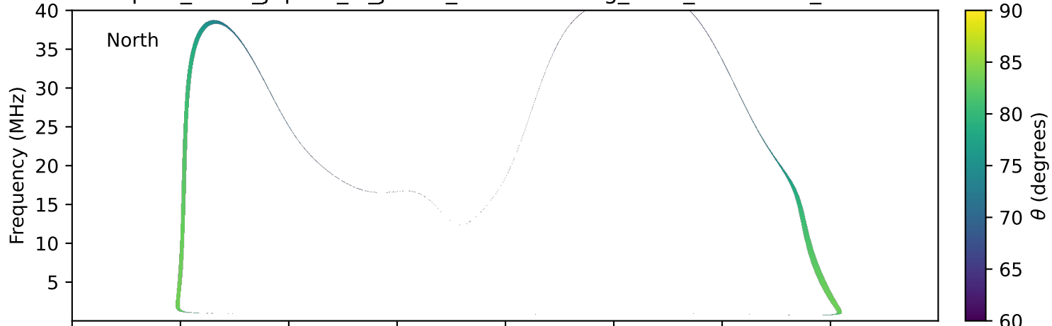
expres_earth_jupiter_io_jrm33_lossc-wid1deg_3kev_20020224_v11.cdf
