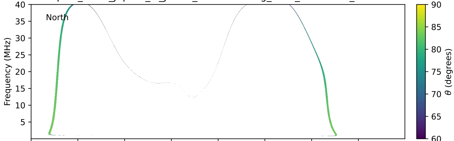
expres_earth_jupiter_io_jrm33_lossc-wid1deg_3kev_20020217_v11.cdf
