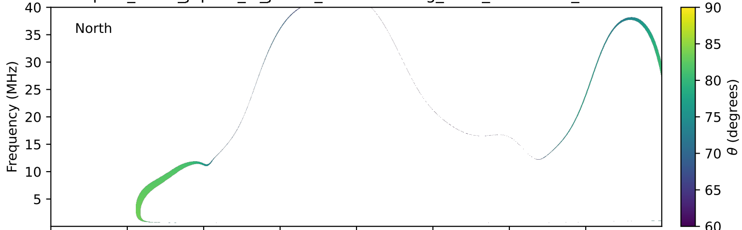
expres_earth_jupiter_io_jrm33_lossc-wid1deg_3kev_20020208_v11.cdf
