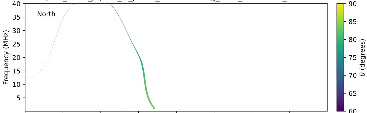
expres_earth_jupiter_io_jrm33_lossc-wid1deg_3kev_20020205_v11.cdf
