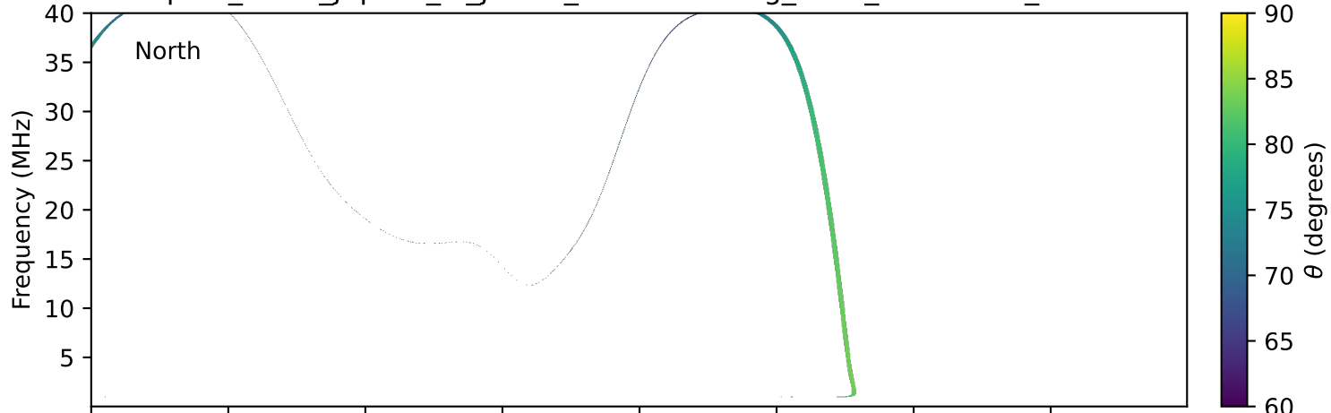
expres_earth_jupiter_io_jrm33_lossc-wid1deg_3kev_20020203_v11.cdf
