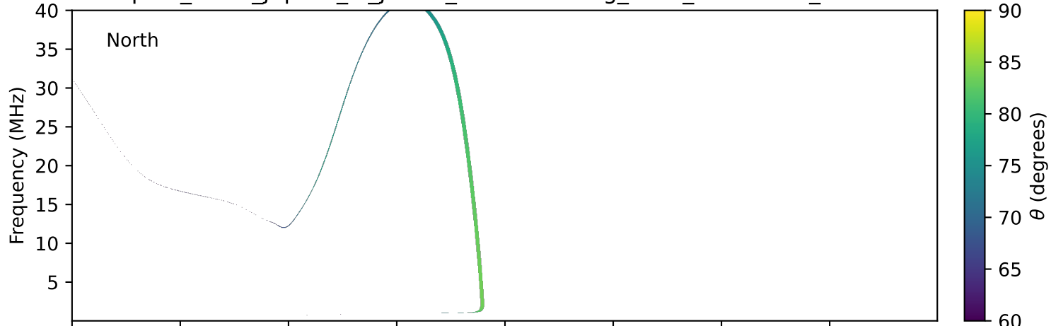
expres_earth_jupiter_io_jrm09_lossc-wid1deg_3kev_20020228_v11.cdf
