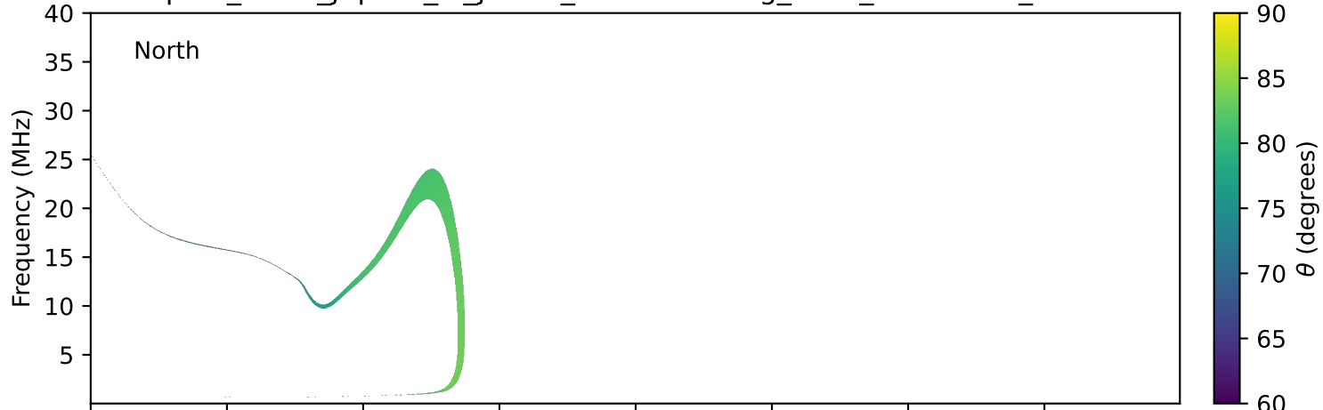
expres_earth_jupiter_io_jrm09_lossc-wid1deg_3kev_20020214_v11.cdf
