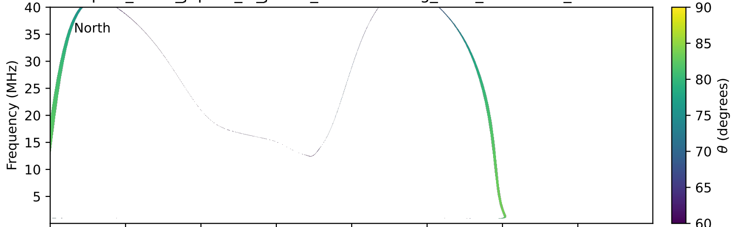
expres_earth_jupiter_io_jrm09_lossc-wid1deg_3kev_20020210_v11.cdf
