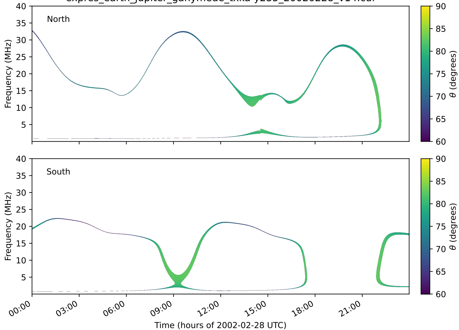
expres_earth_jupiter_ganymede_txka-y235_20020228_v14.cdf
