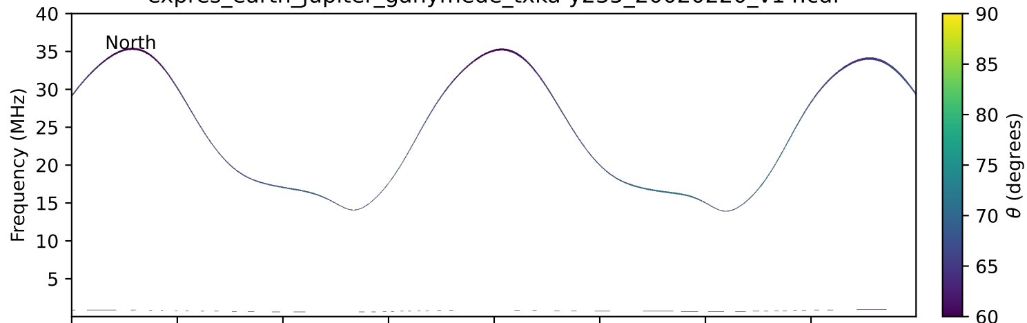
expres_earth_jupiter_ganymede_txka-y235_20020220_v14.cdf
