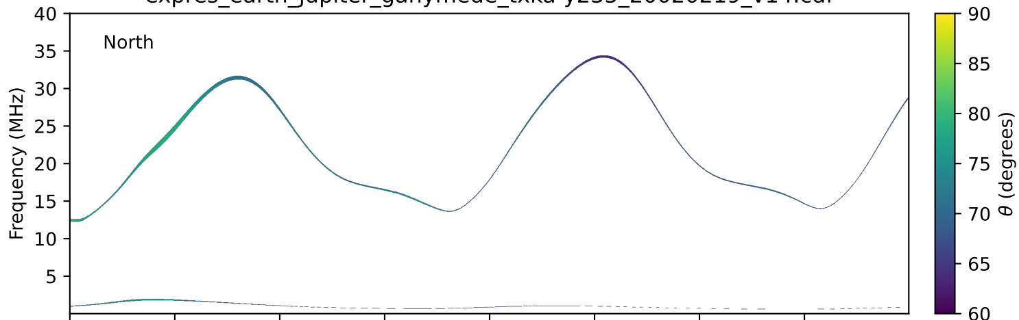
expres_earth_jupiter_ganymede_txka-y235_20020219_v14.cdf
