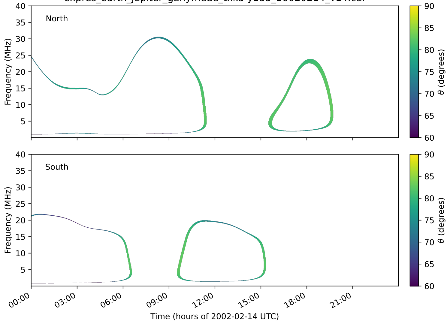
expres_earth_jupiter_ganymede_txka-y235_20020214_v14.cdf
