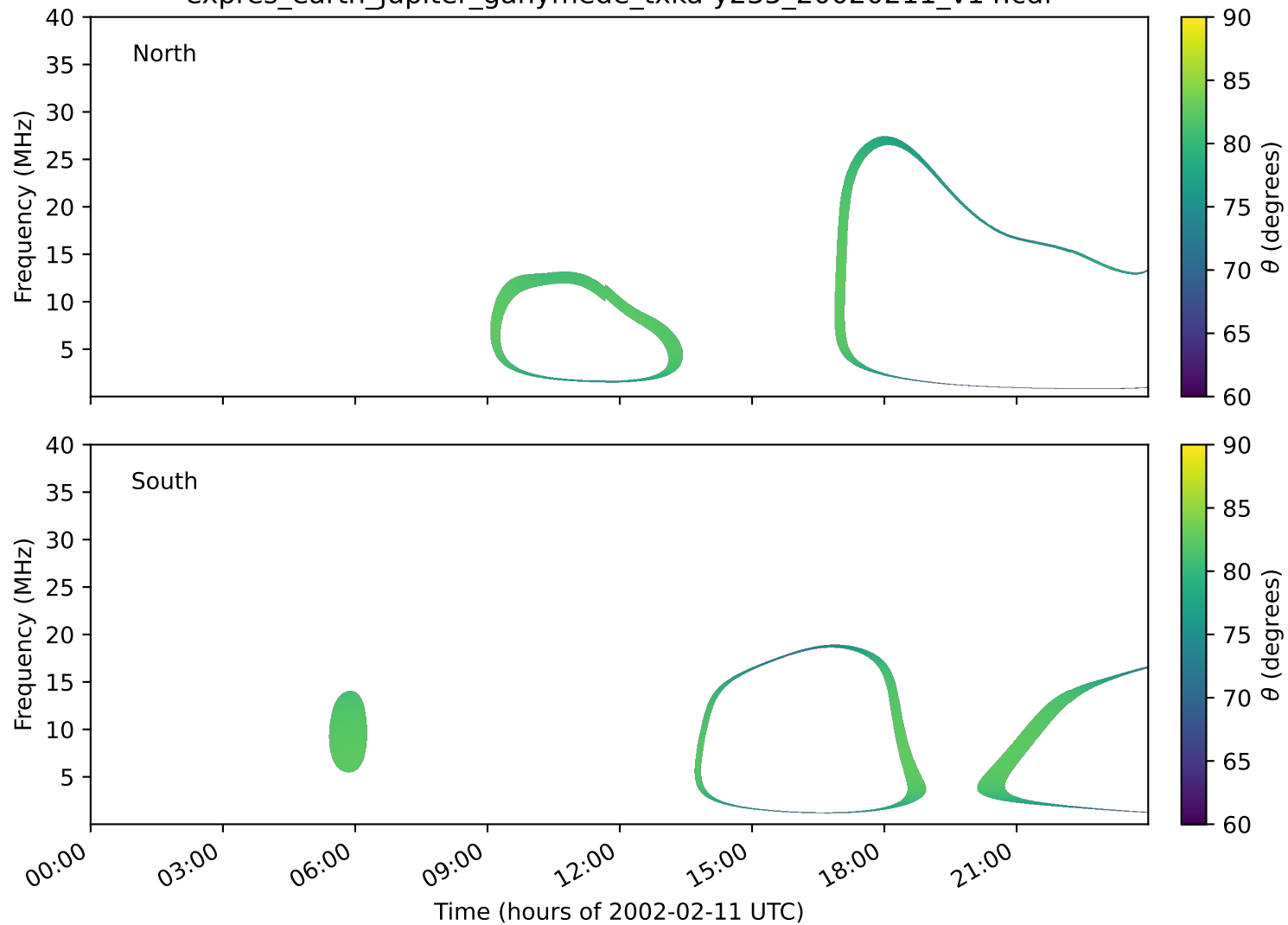
expres_earth_jupiter_ganymede_txka-y235_20020211_v14.cdf
