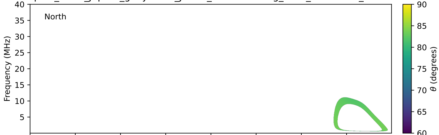
expres_earth_jupiter_ganymede_jrm33_lossc-wid1deg_3kev_20020225_v11.cdf
