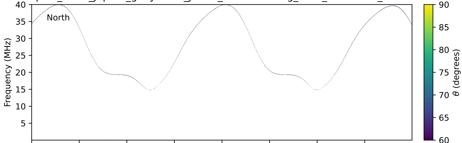
expres_earth_jupiter_ganymede_jrm33_lossc-wid1deg_3kev_20020220_v11.cdf
