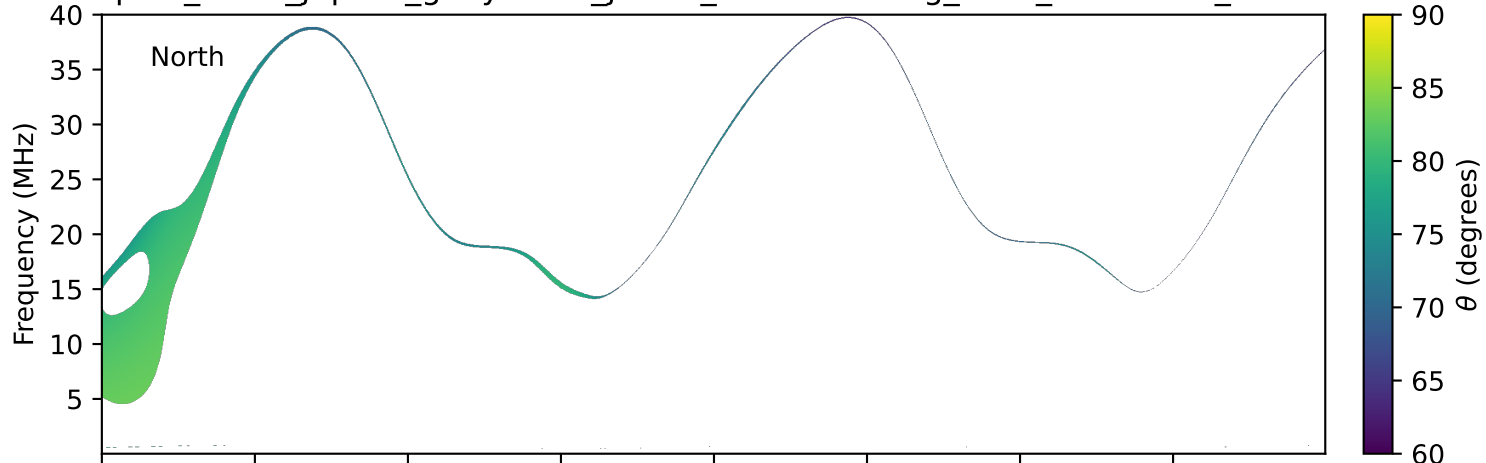
expres_earth_jupiter_ganymede_jrm33_lossc-wid1deg_3kev_20020212_v11.cdf
