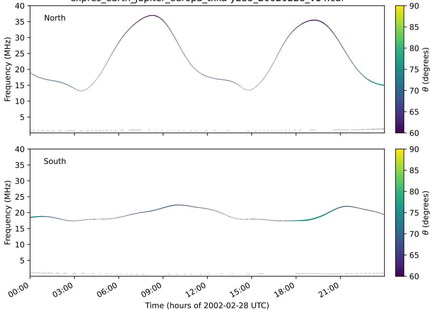
expres_earth_jupiter_europa_txka-y235_20020228_v14.cdf
