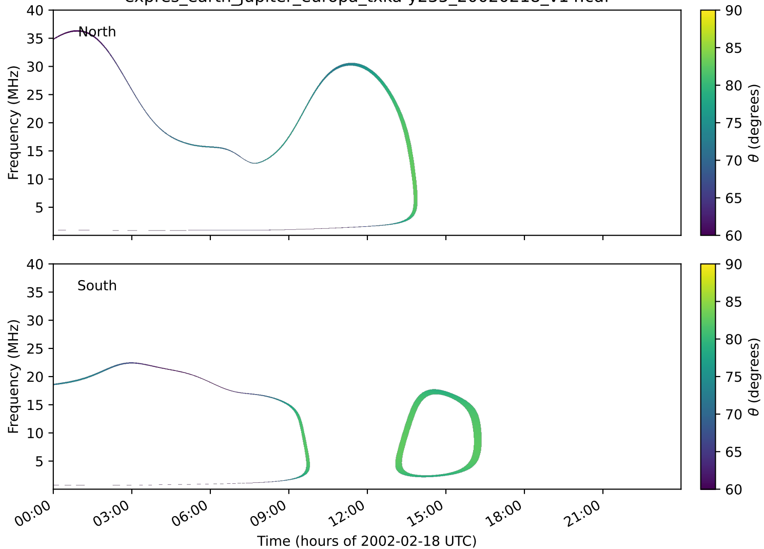
expres_earth_jupiter_europa_txka-y235_20020218_v14.cdf
