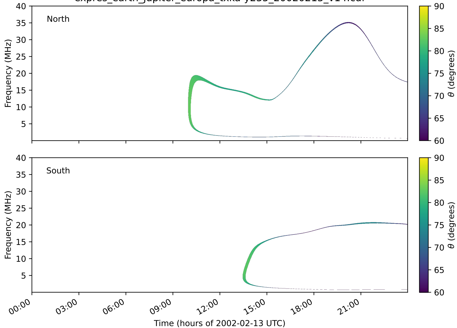
expres_earth_jupiter_europa_txka-y235_20020213_v14.cdf
