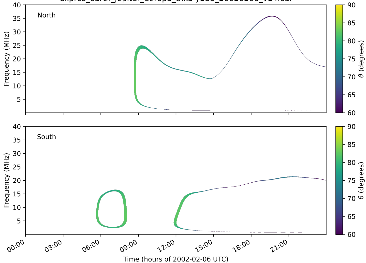
expres_earth_jupiter_europa_txka-y235_20020206_v14.cdf
