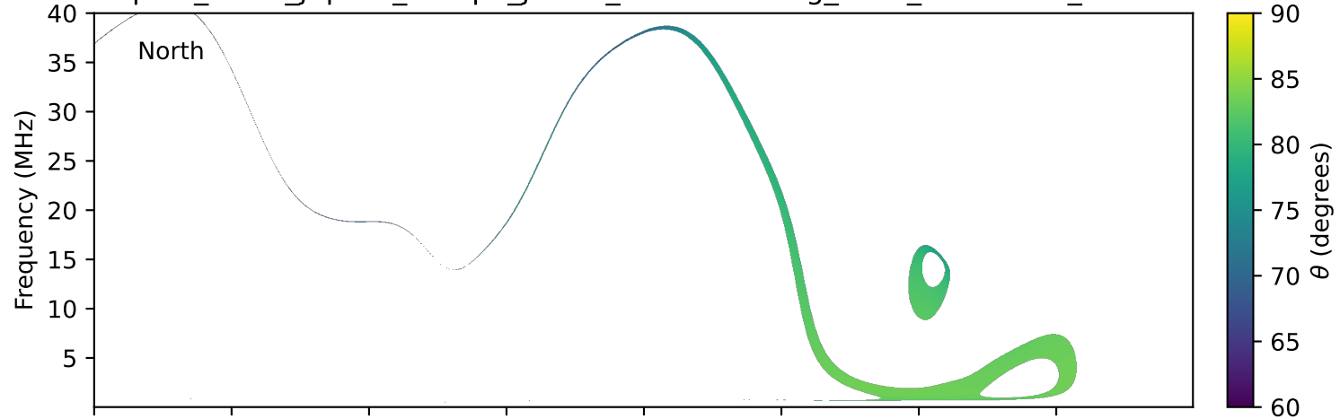
expres_earth_jupiter_europa_jrm33_lossc-wid1deg_3kev_20020225_v11.cdf
