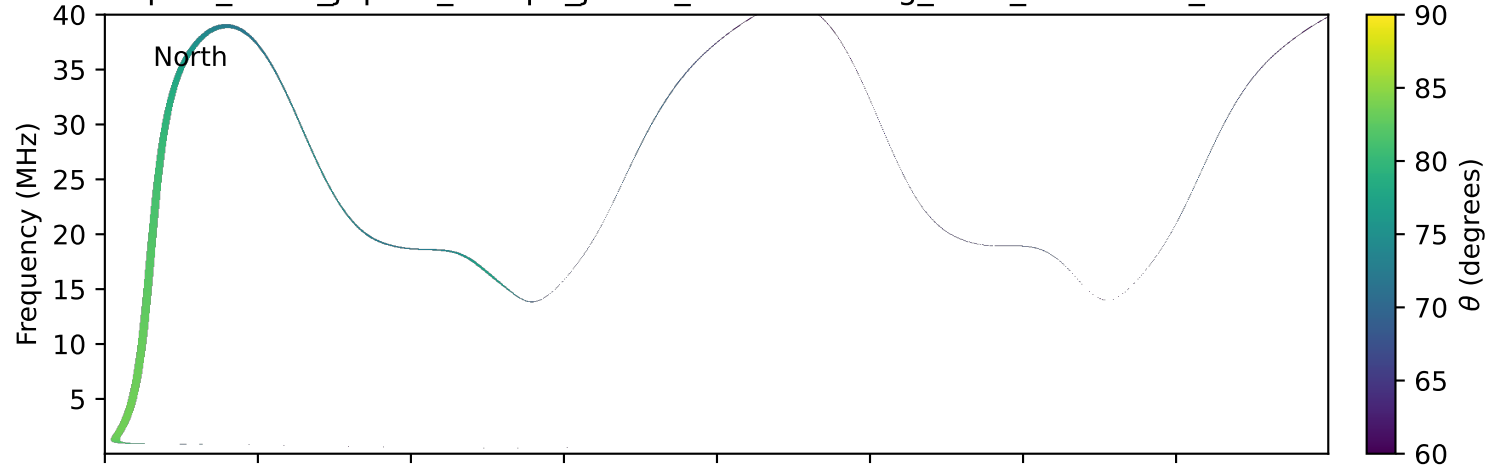
expres_earth_jupiter_europa_jrm33_lossc-wid1deg_3kev_20020210_v11.cdf
