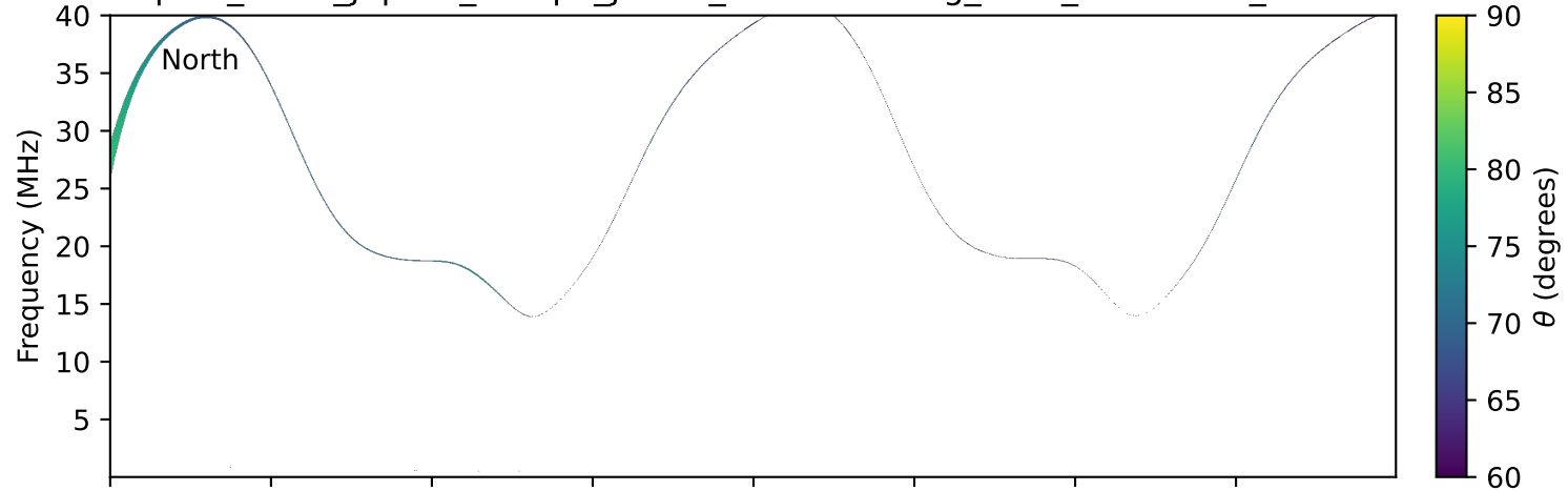
expres_earth_jupiter_europa_jrm33_lossc-wid1deg_3kev_20020203_v11.cdf
