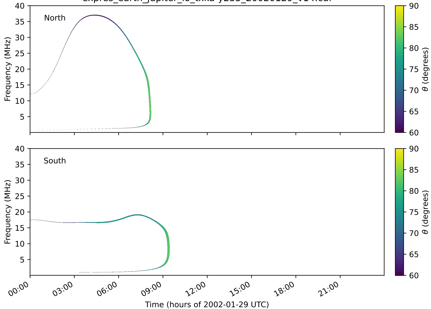
expres_earth_jupiter_io_txka-y235_20020129_v14.cdf
