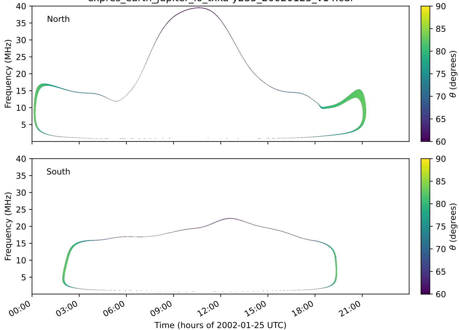
expres_earth_jupiter_io_txka-y235_20020125_v14.cdf
