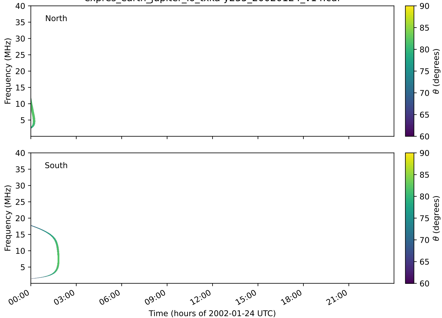
expres_earth_jupiter_io_txka-y235_20020124_v14.cdf
