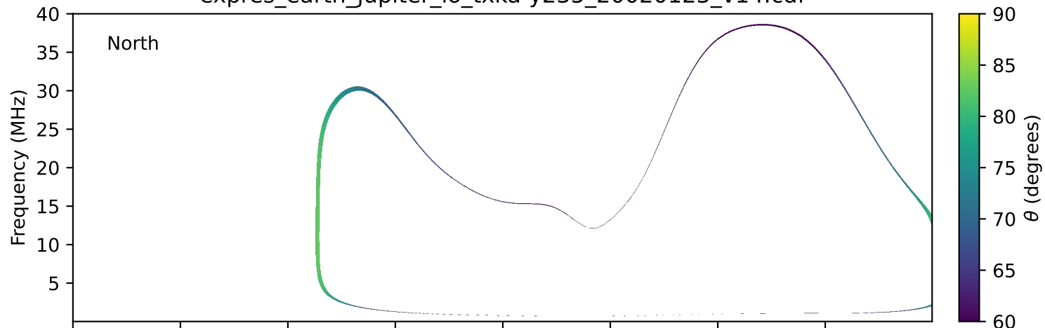
expres_earth_jupiter_io_txka-y235_20020123_v14.cdf
