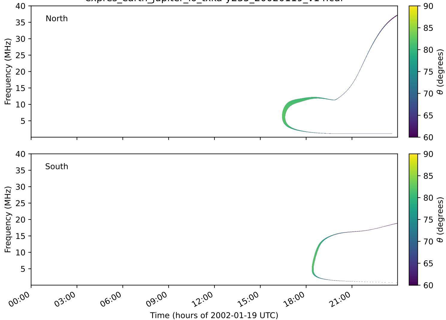
expres_earth_jupiter_io_txka-y235_20020119_v14.cdf
