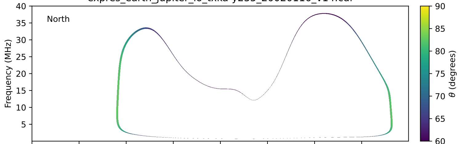
expres_earth_jupiter_io_txka-y235_20020116_v14.cdf
