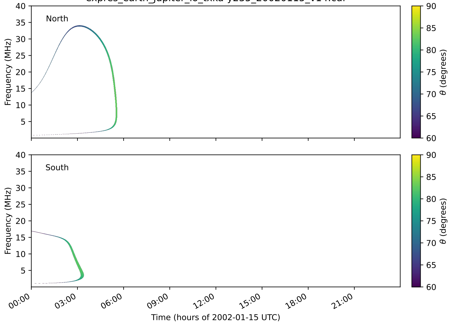
expres_earth_jupiter_io_txka-y235_20020115_v14.cdf
