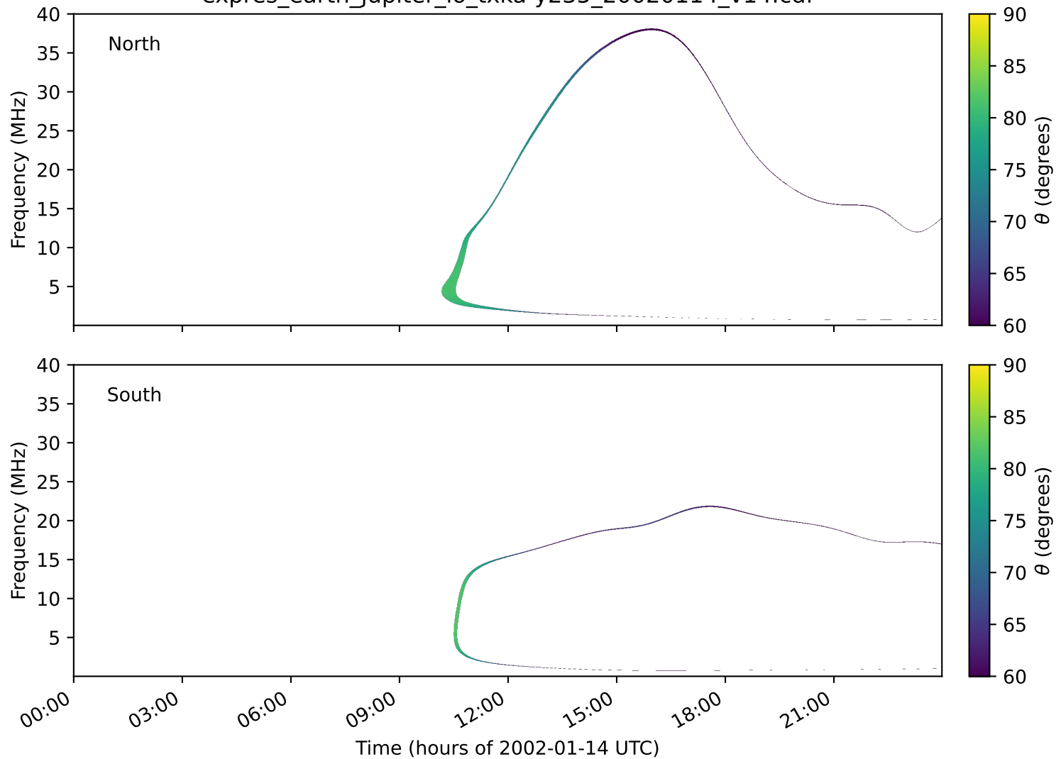
expres_earth_jupiter_io_txka-y235_20020114_v14.cdf
