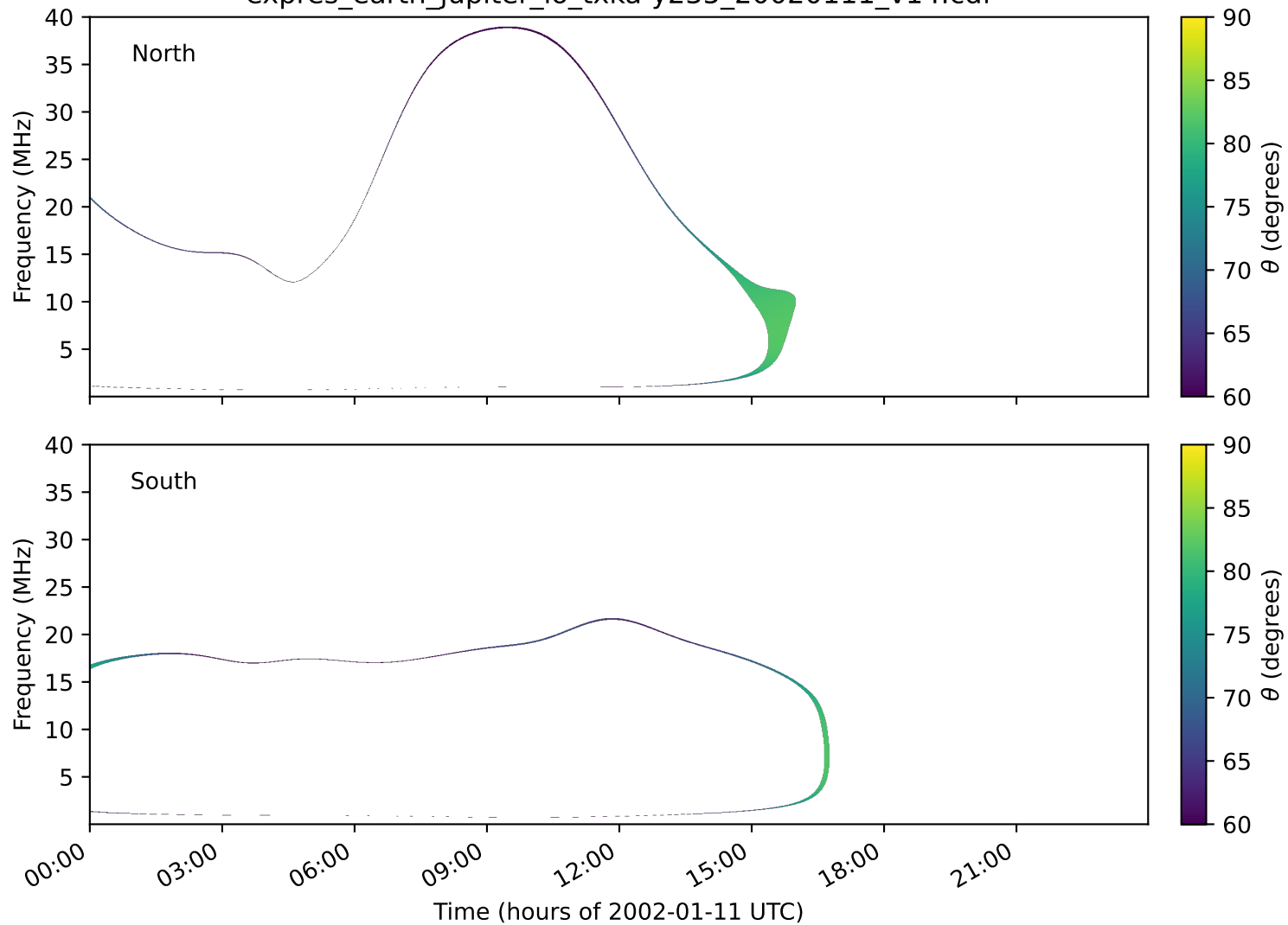
expres_earth_jupiter_io_txka-y235_20020111_v14.cdf
