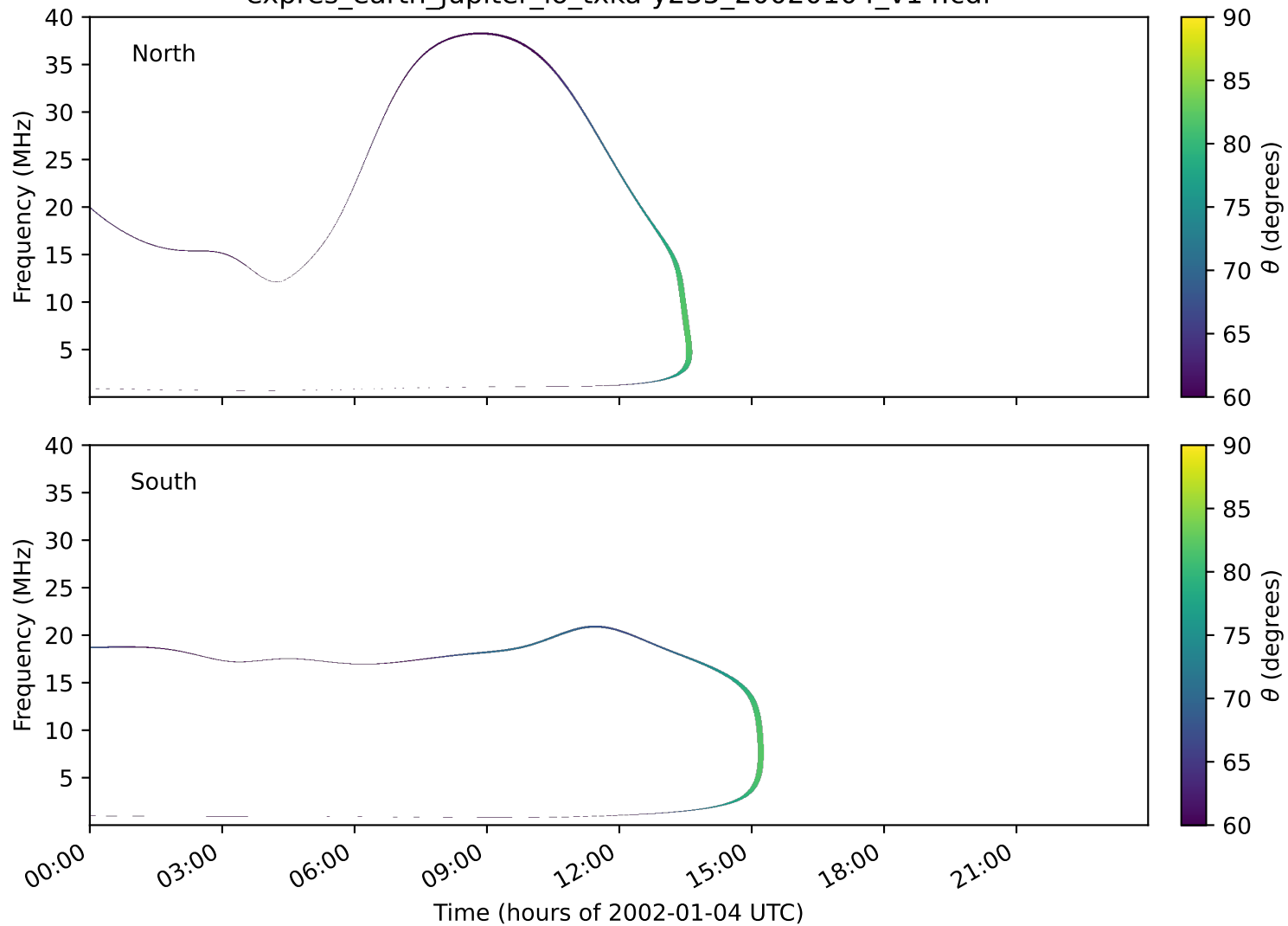
expres_earth_jupiter_io_txka-y235_20020104_v14.cdf
