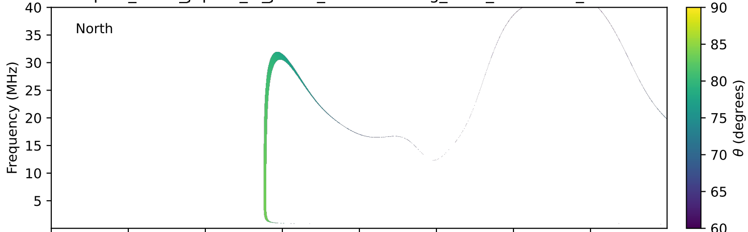
expres_earth_jupiter_io_jrm33_lossc-wid1deg_3kev_20020130_v11.cdf
