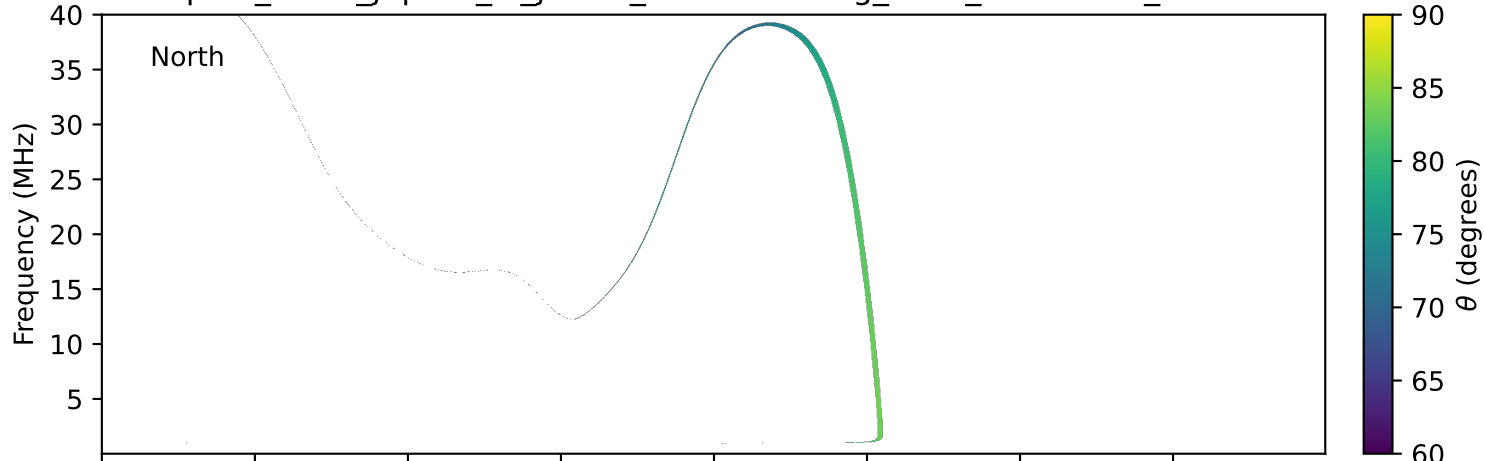
expres_earth_jupiter_io_jrm33_lossc-wid1deg_3kev_20020127_v11.cdf
